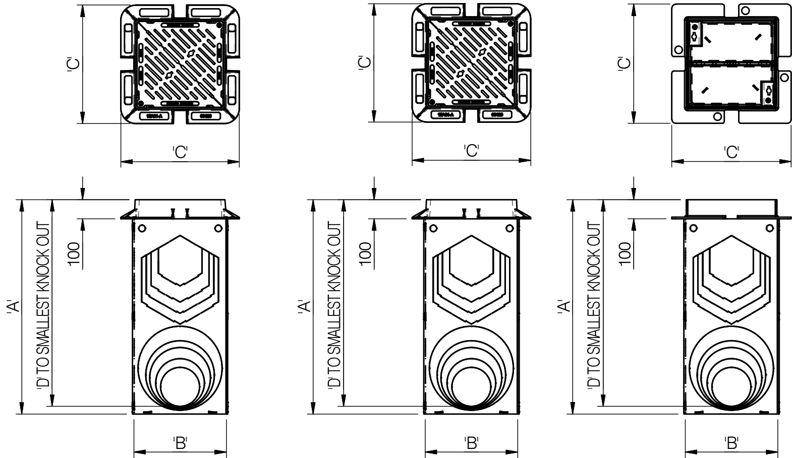
GATIC OUTLET BOX WITH F900 DOUBLE TRIANGULAR GRATING
